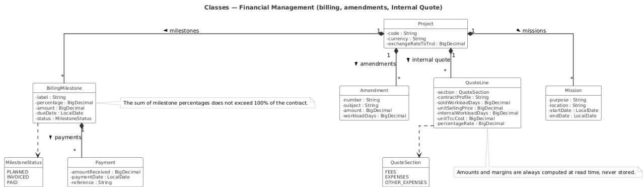
FIGURE 6.1 : Class diagram — financial management
