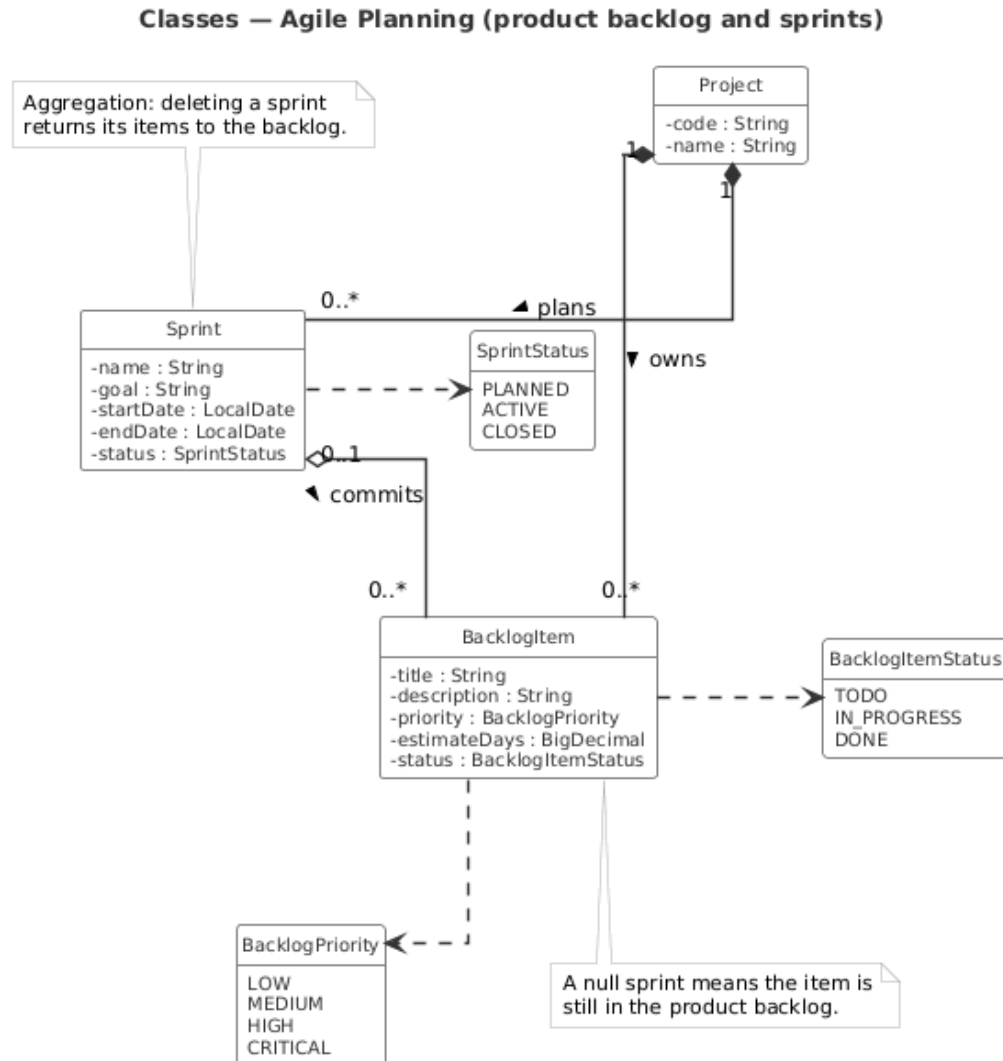
FIGURE 5.7 : Class diagram — agile planning
