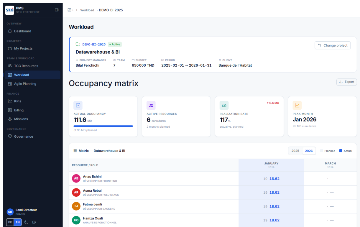
FIGURE 5.6 : Workload matrix interface
