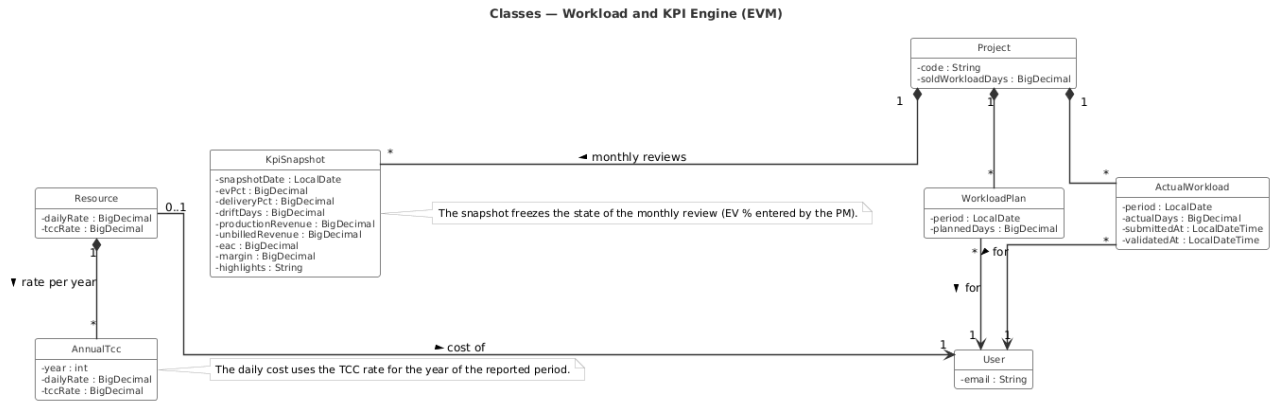
FIGURE 6.5 : Class diagram — workload and indicator engine
