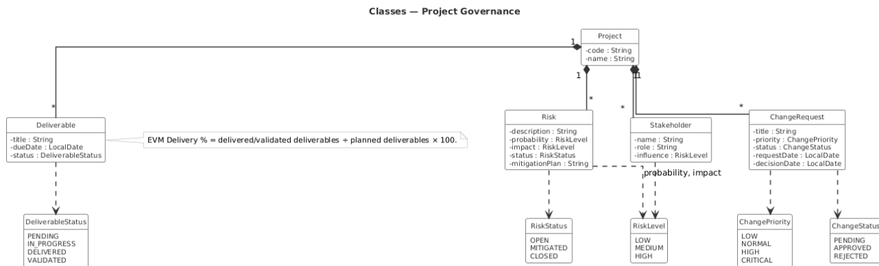
FIGURE 6.3 : Class diagram — project governance
