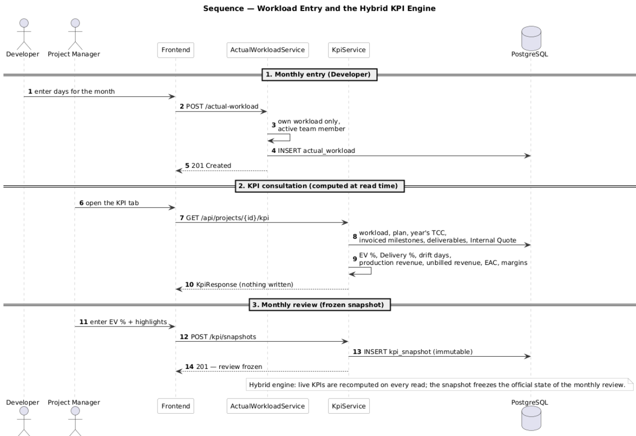
FIGURE 6.6 : Sequence diagram — workload entry and indicator computation
