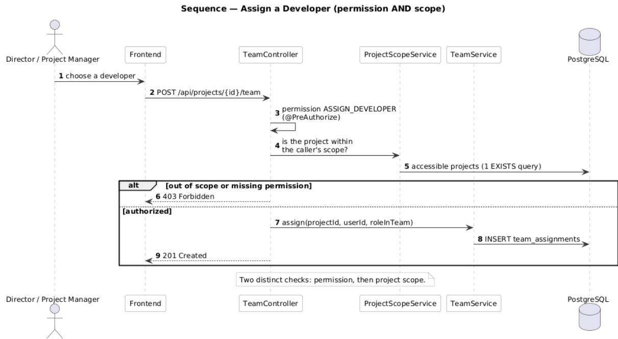
FIGURE 5.5 : Sequence diagram of the “Assign a developer” use case
